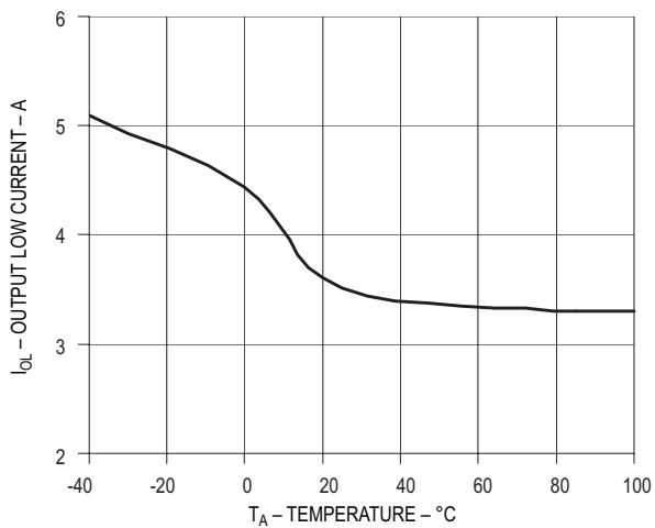
Figure 5. I_{OL} vs. Temperature
