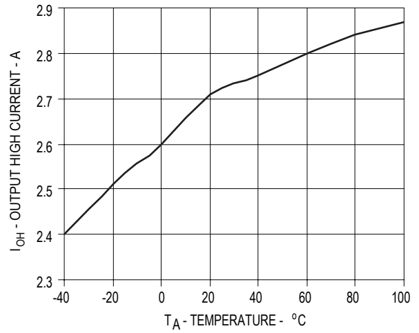
Figure 2. I_{OH} vs. Temperature
