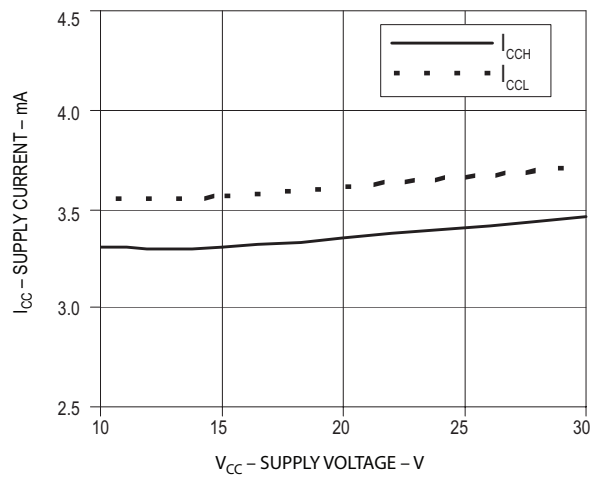
Figure 8. I_{CC} vs. V_{CC}
