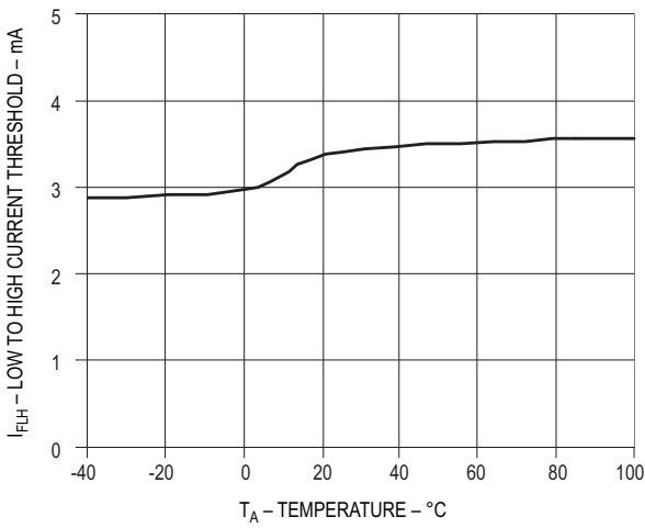
Figure 9. I_{FLH} vs. Temperature
