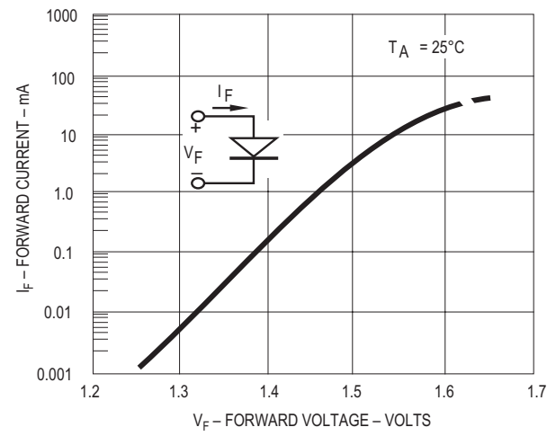
Figure 16. Input Current vs. Forward Voltage
