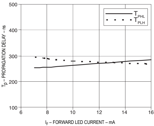
Figure 11. Propagation delay vs. I_F
