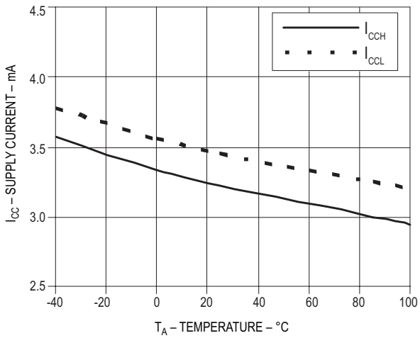
Figure 7. I_{CC} vs. Temperature
