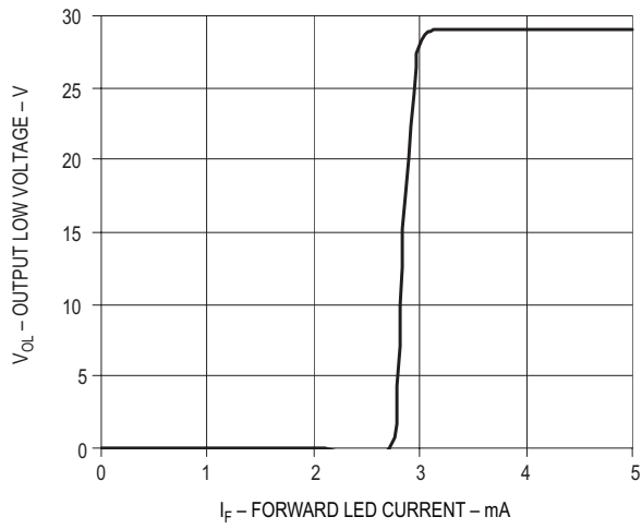
Figure 15. Transfer Characteristics
