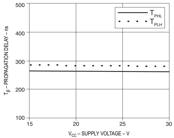
Figure 10. Propagation delay vs. V_{CC}
