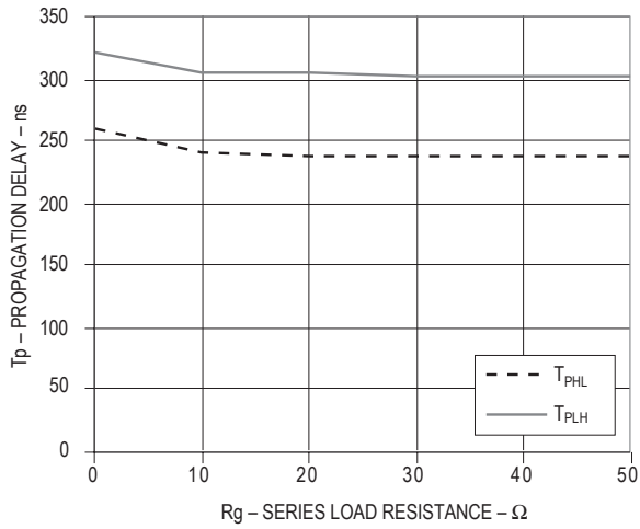
Figure 13. Propagation Delay vs. Rg
