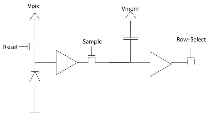
Figure 4. 6T-pixel architecture
